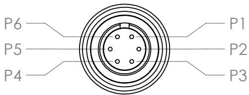
CONNECTOR SHOW FROM THE REAR (TERMINATION) SIDE
